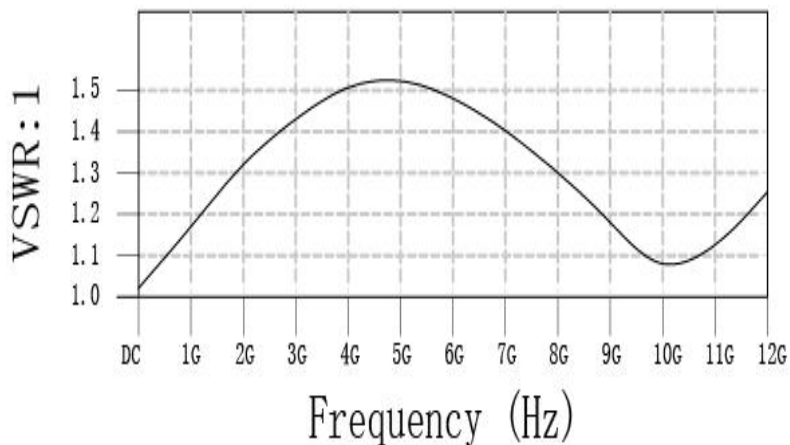
典型VSWR, 25°C
