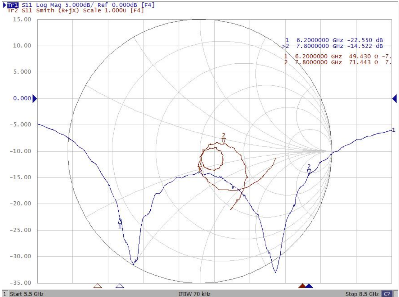
Return loss
