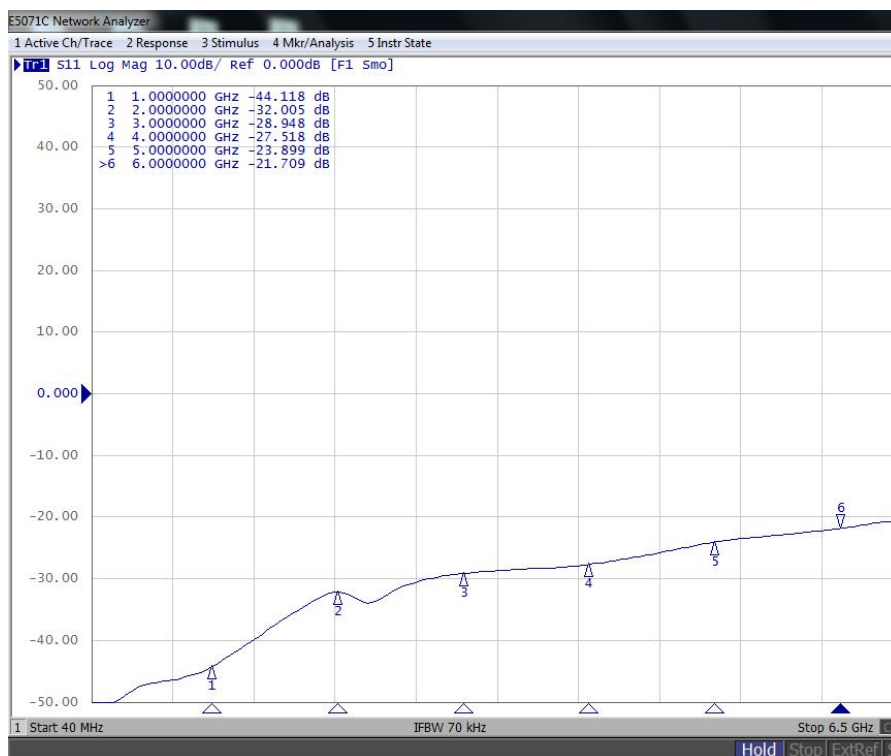
Retrun Loss
