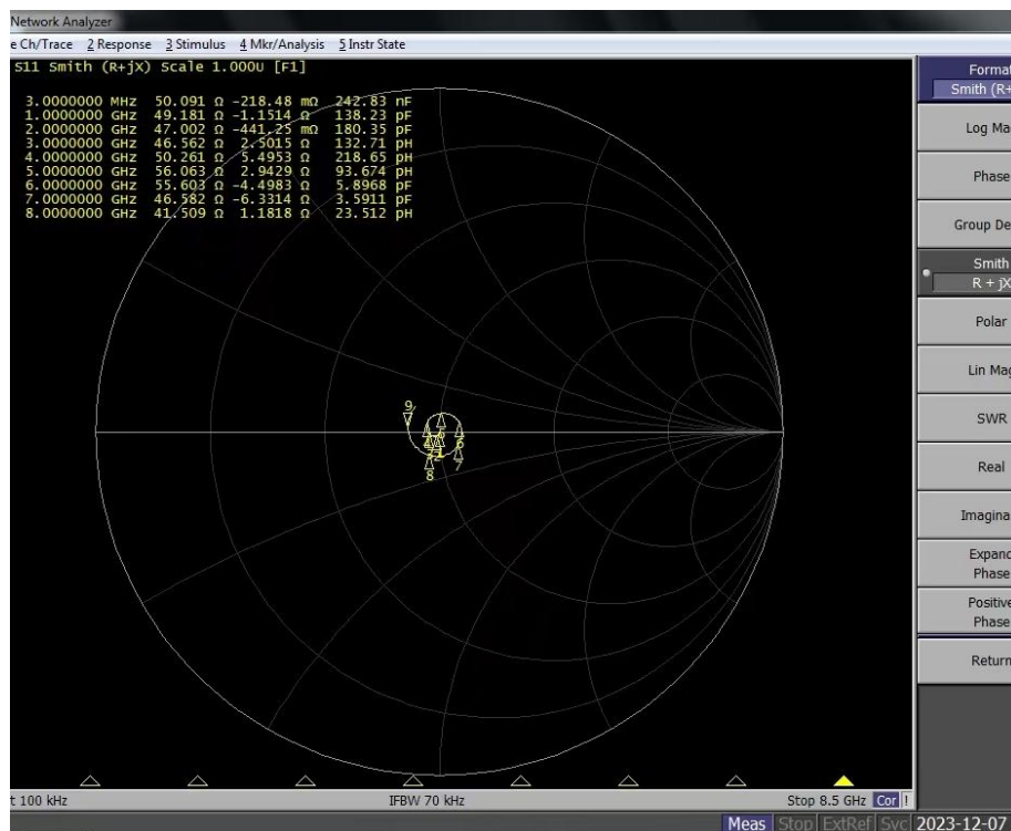
Smith Chart
